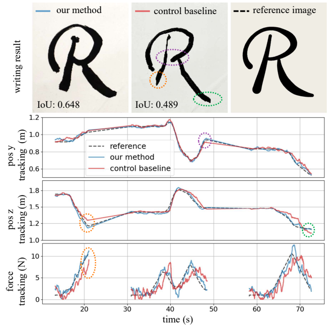
Fig. 6. Comparison with the control baseline. Top: Writing results for letter ‘R’. Bottom: Time history of end-effector motion and contact force tracking performance.
